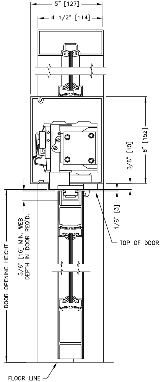
SECTION: 2
