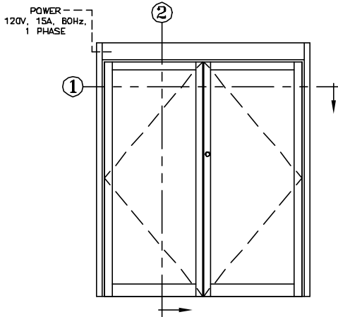
ELEVATION VIEW
